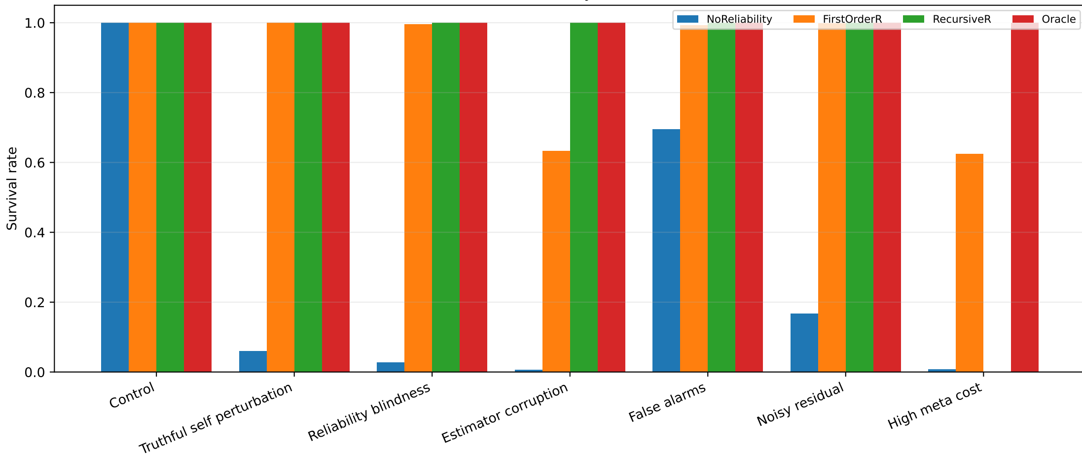
Survival rate by condition
